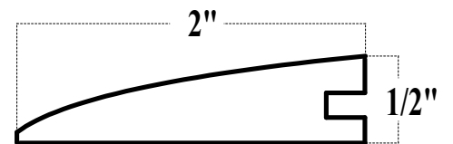
1/2" Flush Reducer
