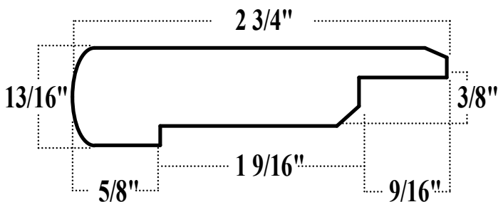
Overlap Stairnose
