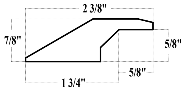
Overlap Reducer
