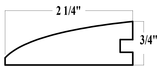
3/4" Flush Reducer
