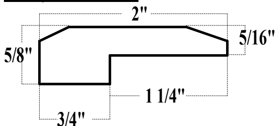
Baby-Treshold
